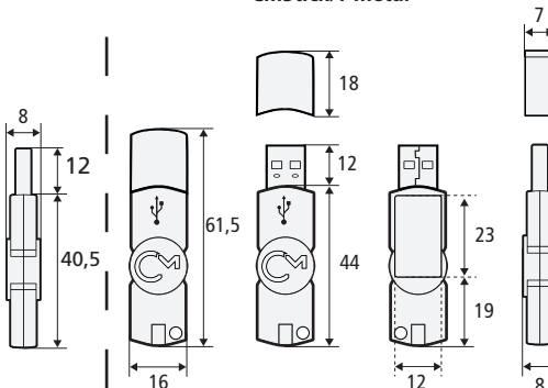
CmStick/T metal
