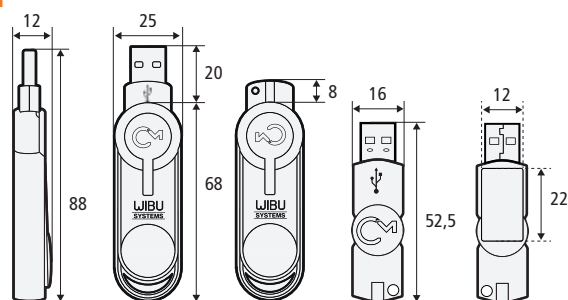
CmStick/T plastic
